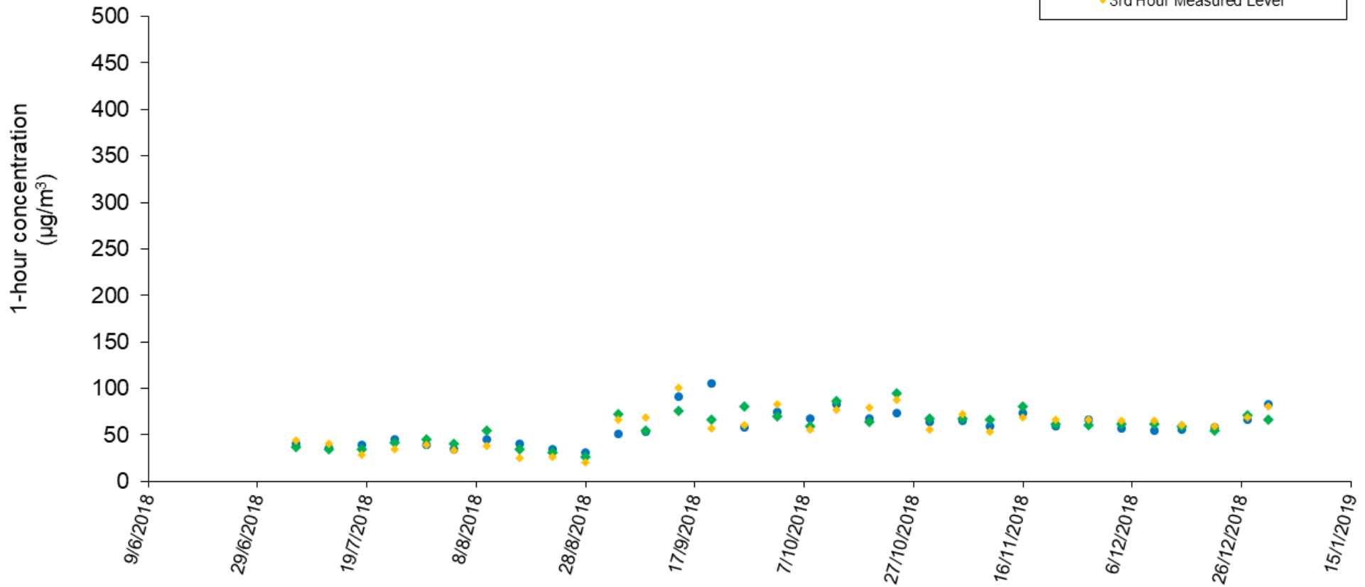
1-hour TSP concentration vs date for Location W-A6
