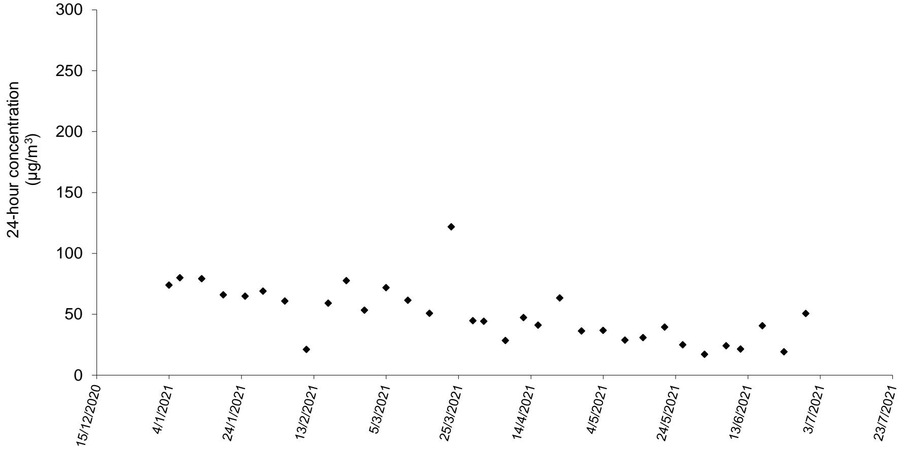
24-hour TSP concentration vs date for Location E-A1
